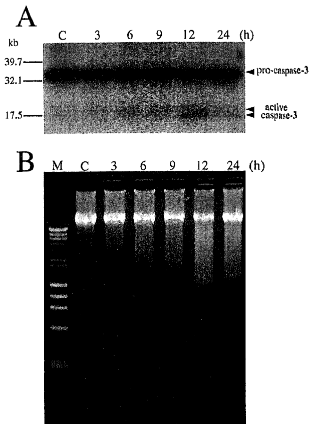
Figure 5. Caspase-3 activation examined by Western blot analysis (A) and induction of nucleosomal DNA fragmentation (B) after treatment with 10 \mu M \alpha -mangostin in HL60 cells. Lane M is a DNA size marker. C, control. The periods of treatment are indicated in each lane.
