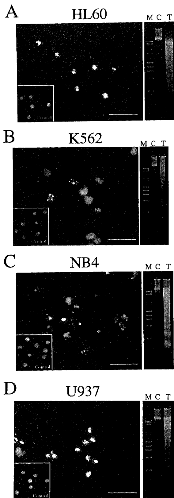
Figure 4. \alpha -Mangostin-induced apoptosis in human leukemia cell lines HL60 (A), K562 (B), NB4 (C), and U937 (D) treated at 10 \mu M for 24 h. Morphological examination was performed by Hoechst 33342 staining ( \times 400 , bar = 50 \mu m). The films of untreated control cells were inserted into the left corners in contrast with treated cells. Nucleosomal DNA fragmentation detected by agarose gel electrophoresis in each cell line was also demonstrated (M, DNA size marker; C, control; T, \alpha -mangostin-treated cells).
