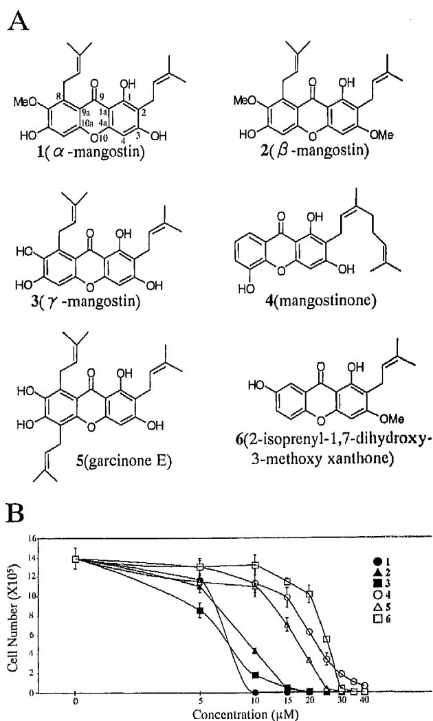
Figure 1. Chemical structure of xanthenes (A) and effects of xanthenes on concentration-dependent cell growth inhibition in HL60 cells at 72 h after treatment (B). Starting cell number is 1 \times 10^5/m . Data are expressed as means \pm SD of three different experiments.
