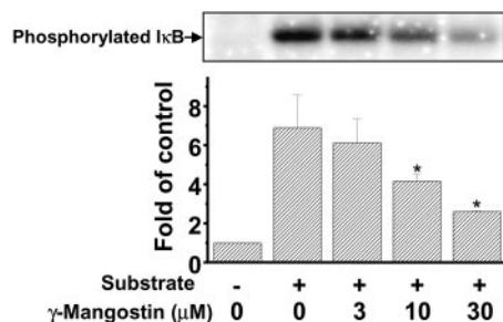
Fig. 5. Concentration-dependent inhibitory effect of \gamma -mangostin on IKK activity. C6 cells were harvested, lysed, and immunoprecipitated with anti-IKK \alpha/\beta antibody. The kinase assay was carried out in 25 \mu l of kinase buffer containing 5 \mu M ATP, 10 \mu Ci [ \gamma - 32 P]ATP (5000 Ci/mmol), and 1 \mu g I \kappa B \alpha (1–317) as a substrate and incubated with the indicated concentrations of \gamma -mangostin at 25°C for 30 min. The samples were subjected to SDS-PAGE (11% gel). At the top is a representative radioluminogram detected by using a molecular imager (GS363; Bio-Rad). At the bottom, data obtained by densitometry are shown. The results are shown as the fold increase from the value for a sample excluding the substrate and \gamma -mangostin (0.1% DMSO alone). Each column represents the mean \pm S.E.M. ( n = 3 ). *, P < 0.05 compared with the value for the sample containing the substrate but not \gamma -mangostin (as vehicle control).
