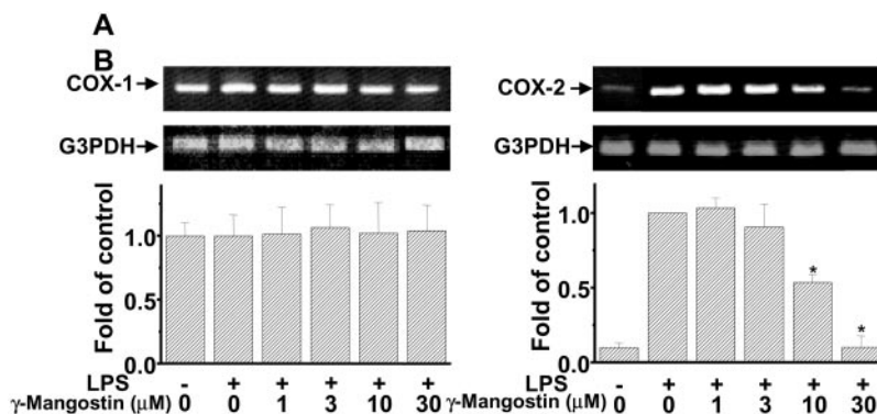
Fig. 4. Decreasing effects of \gamma -mangostin on COX-1 (A) and COX-2 (B) mRNA expression in C6 cells as measured by RT-PCR. Cells were preincubated with the indicated concentrations of \gamma -mangostin or without this compound for 1 h and thereafter were incubated in the absence or presence of 10 \mu g/ml LPS for 1 h. Total RNA from C6 cells was used as a template for cDNA synthesis and then subjected to PCR as described under Materials and Methods . Glyceraldehyde-3-phosphate dehydrogenase mRNA was used as the loading control. Shown are representative expression patterns from three independent experiments (top). The densitometric data on COX-1 and COX-2 mRNA expression (bottom) are calculated as the fold increase of the value for cells not treated with \gamma -mangostin. Each point represents the mean \pm S.E.M. ( n = 3 ). *, P < 0.05 compared with the value for cells treated with 0.1% DMSO (as vehicle control).
