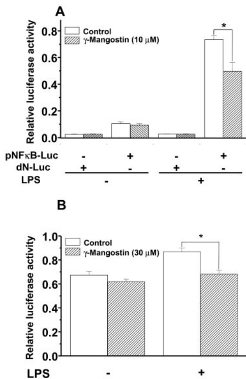
Fig. 7. Inhibitory effect of \gamma -mangostin on LPS-induced enhancement of luciferase activity of pNF \kappa B-Luc (A) or pHES2(-327/+59)-Luc (B) in C6 cells. Cells were transfected with 0.475 \mu g/well pNF \kappa B-Luc or dN-Luc (the NF- \kappa B-responsive element-deficient pNF \kappa B-Luc), or 0.4 \mu g/well pHES2(-327/+59)-Luc, and 0.025 \mu g/well of pRG-TK plasmid. After transfection, cells were preincubated with the indicated concentration of \gamma -mangostin or without this compound for 3 h and then incubated in the absence or presence of 1 \mu g/ml LPS for 8 h. Cells were harvested, and thereafter the luciferase activity was determined as described under Materials and Methods . Relative luciferase activity was calculated as the ratio of firefly luciferase activity to R. reniformis luciferase activity. Each column represents the mean \pm S.E.M. ( n = 3 ). *, P < 0.05 compared with the value for cotransfected cells with pNF \kappa B-Luc (A), or pHES2(-327/+59)-Luc (B) and pRG-TK plasmid, which were treated with LPS alone (0.1% DMSO).
